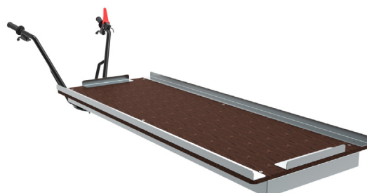
Platform 1500x600 mm A063.701
